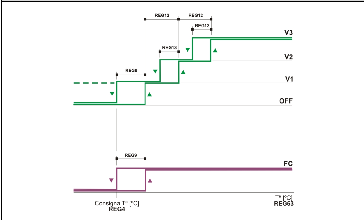
FC: Fan-coil
